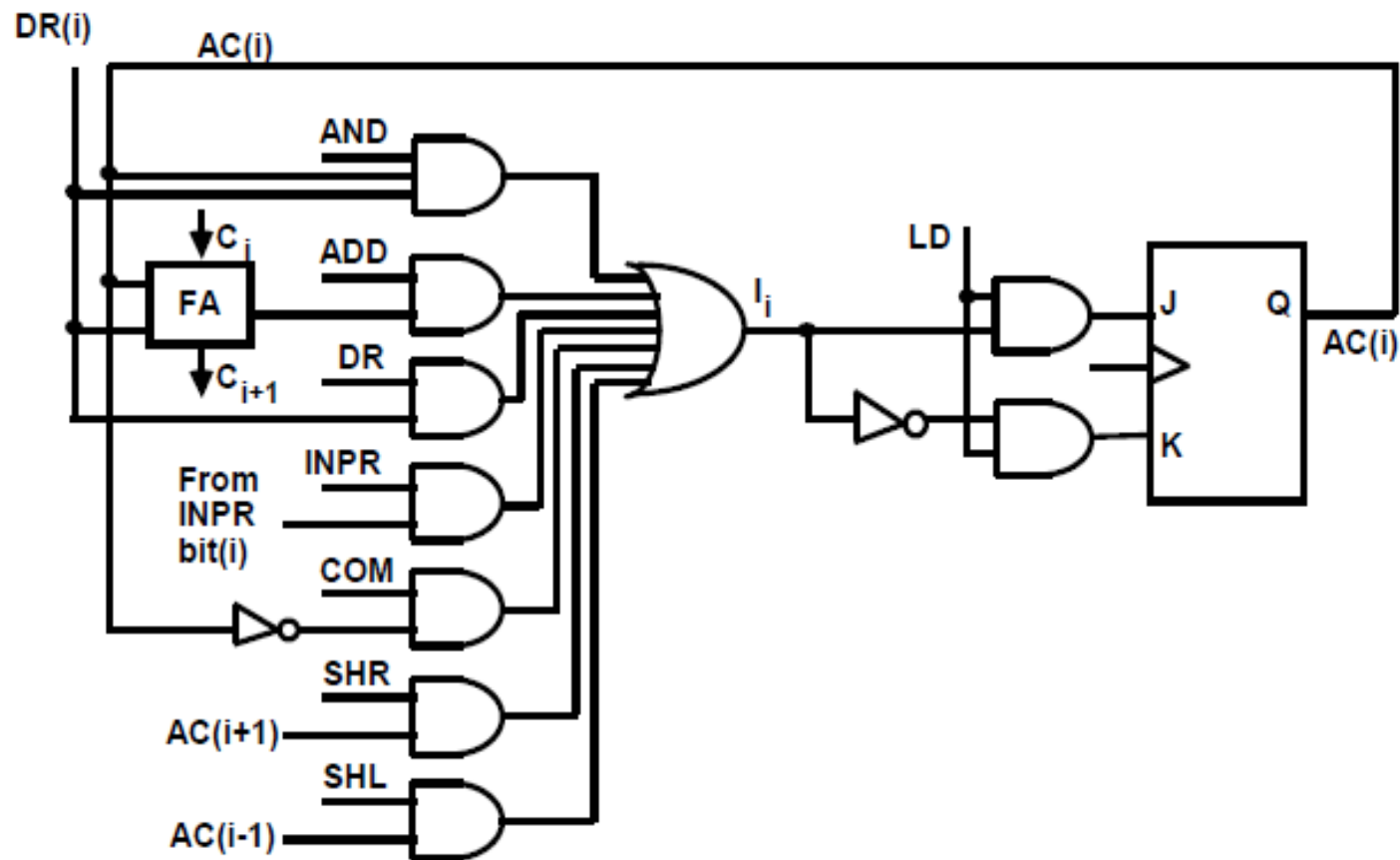
One stage of Adder and Logic circuit
